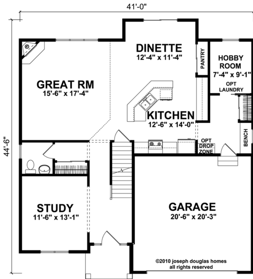
1st Floor 1,222 sq. ft.
