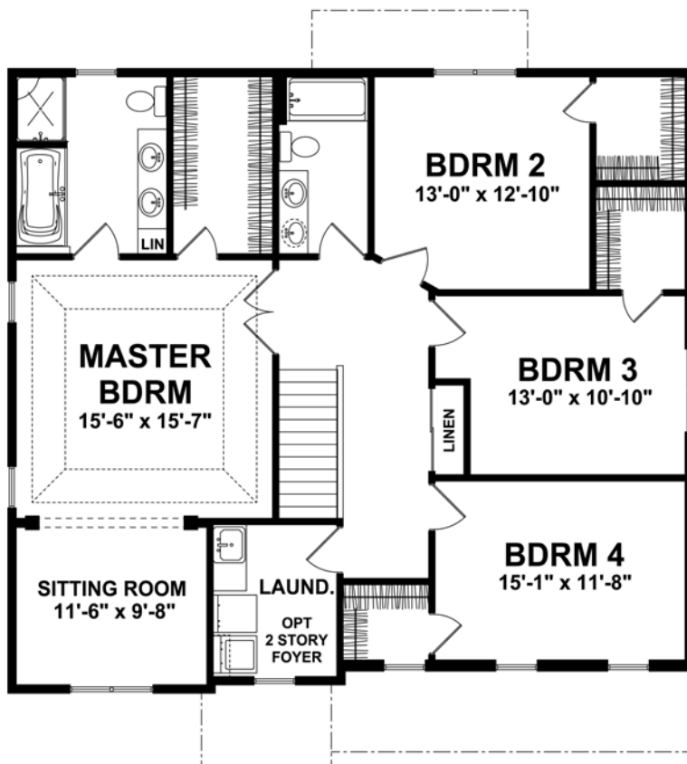
2nd Floor 1,481 sq. ft.
